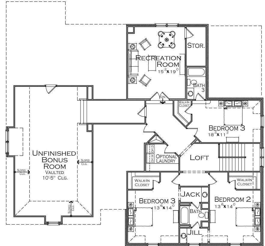
UPPER LEVEL
