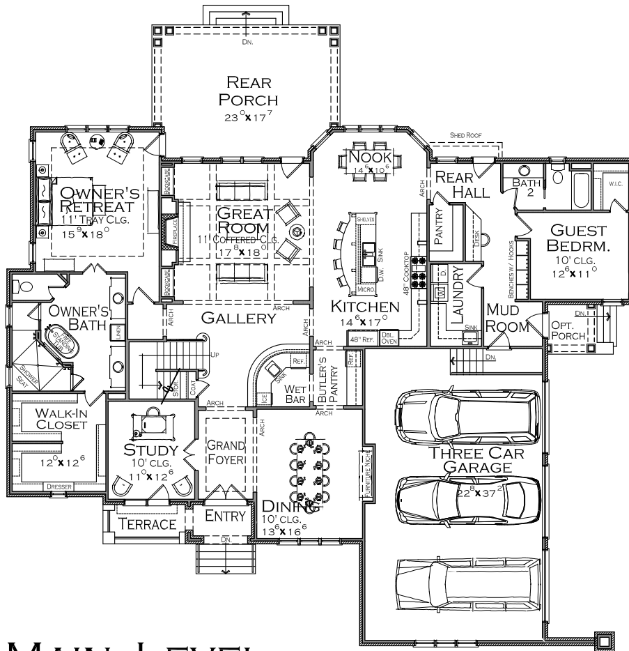
MAIN LEVEL
