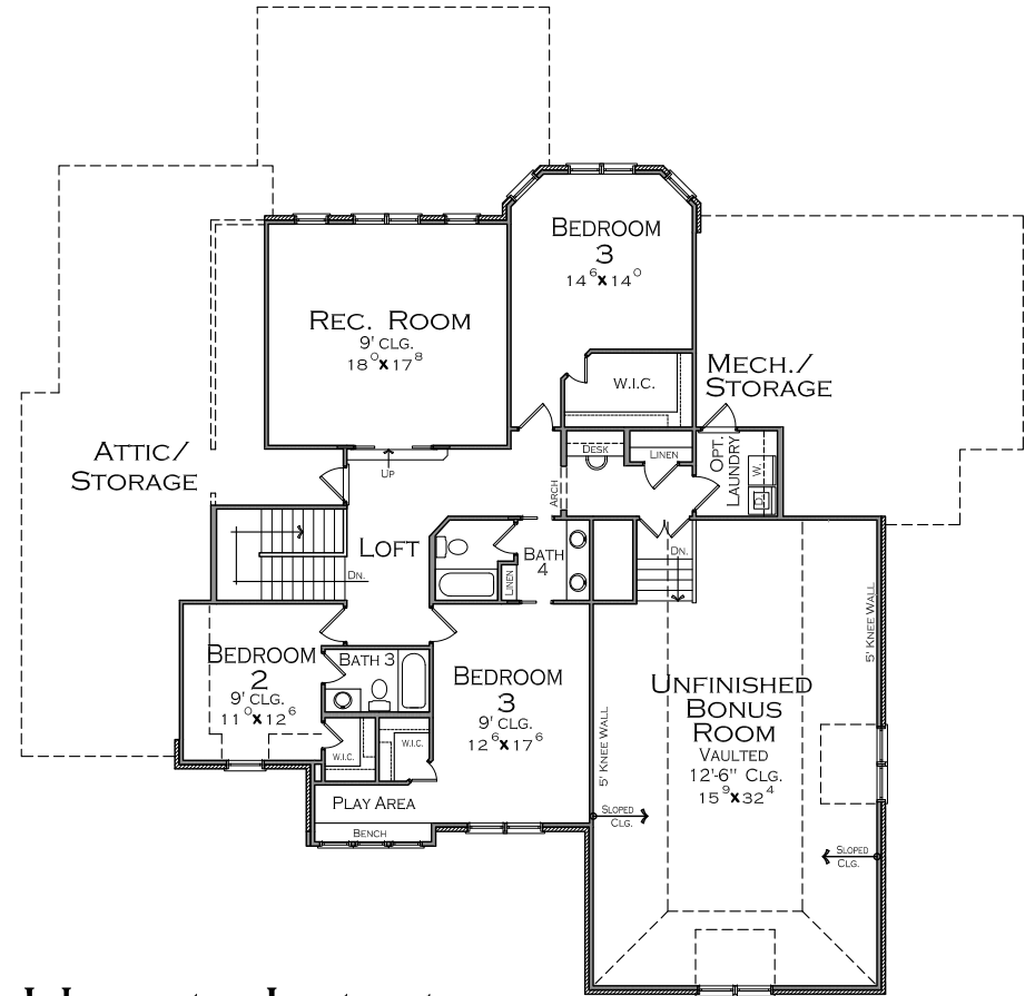
UPPER LEVEL
